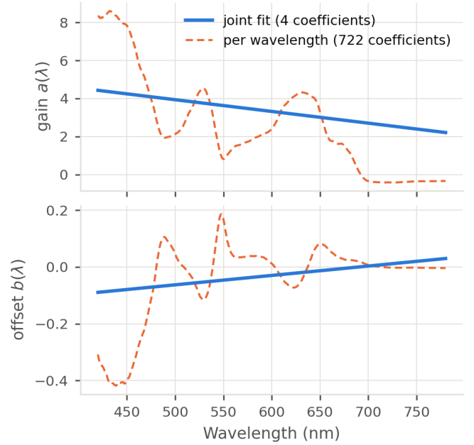
Figure 2. The fitted correction. The per-wavelength fit is free to follow the training samples, while the first-degree joint fit is two straight lines. The constrained model keeps the drift and drops the excursions.
