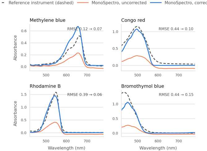
Figure 4. The test set: four laboratory dyes measured in a later session, shown uncorrected, corrected, and as recorded by the reference instrument (dashed).
