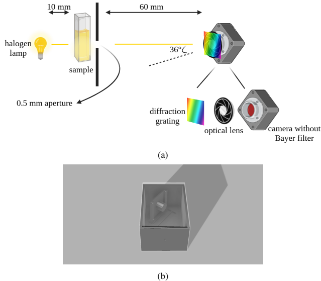
Figure 1. (a) Optical path. Light from the halogen source crosses the cuvette and the entrance slit and is dispersed by a diffraction grating bonded directly to the front face of the lens. The sensor is tilted by 36^\circ so that the first order of the visible band falls across it. (b) The assembled instrument. replace with the hero photograph of the built unit
