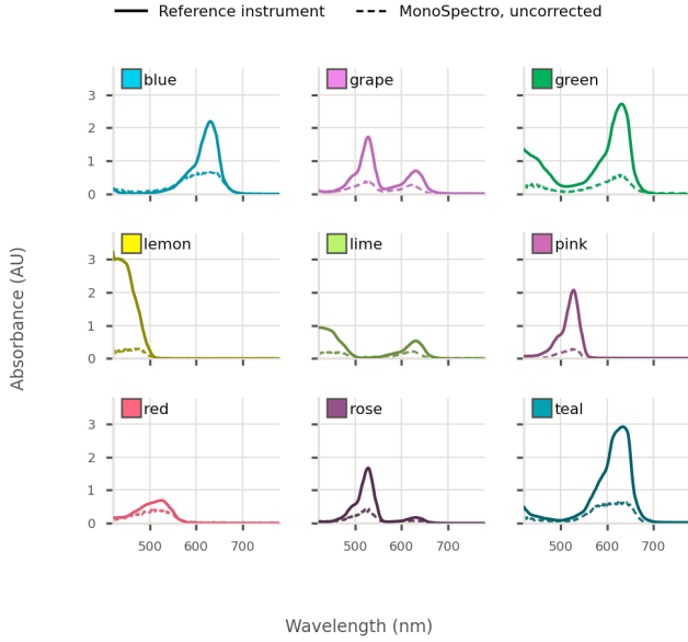
Figure 3. The nine commercial food colourings used to fit the correction, as recorded by the reference instrument and by MonoSpectro before any correction. Each swatch is the solution’s own transmitted colour. The device tracks the position and width of every band but reads systematically low on the absorbance scale, which is the deviation the response function models.
